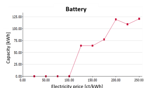
Fig 4. Battery sensitivity analysis.
