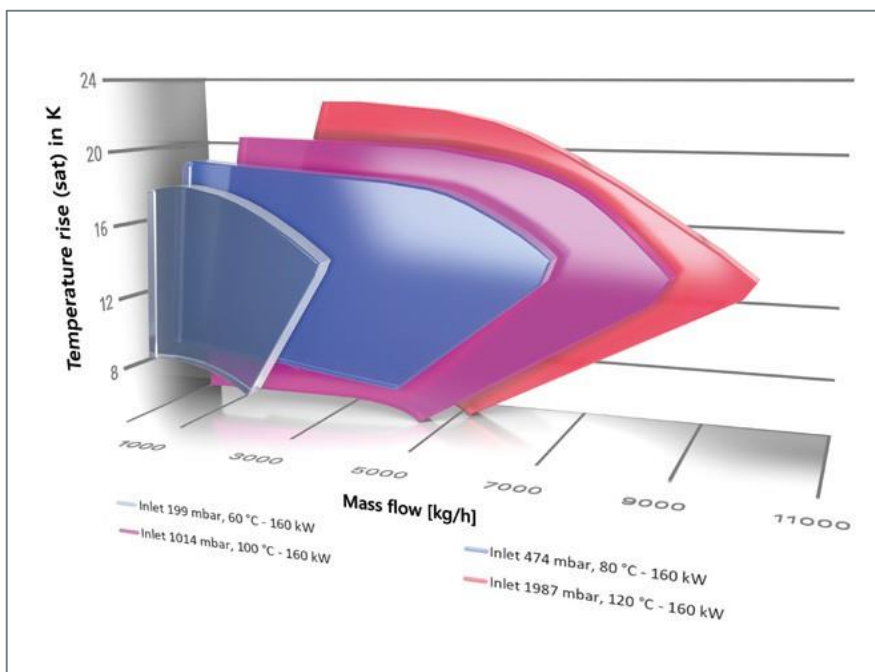
2-stage design - Performance summary of VapoFan product range
